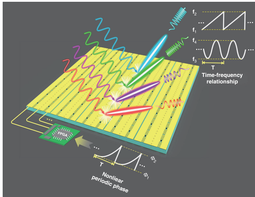
Fig. 1 Concept illustration of waveform generations and beam shaping of various FMCWs by a programmable STCM with nonlinearly periodic phases. Under the control of a FPGA that offers external nonlinear periodic voltage control signals, the different types of FMCW signals can be synthesized as required at the same STCM platform. By further optimizing the initial voltage distributions among different regions of the metasurface, the propagation directions of the FMCW beams can be manipulated freely.
