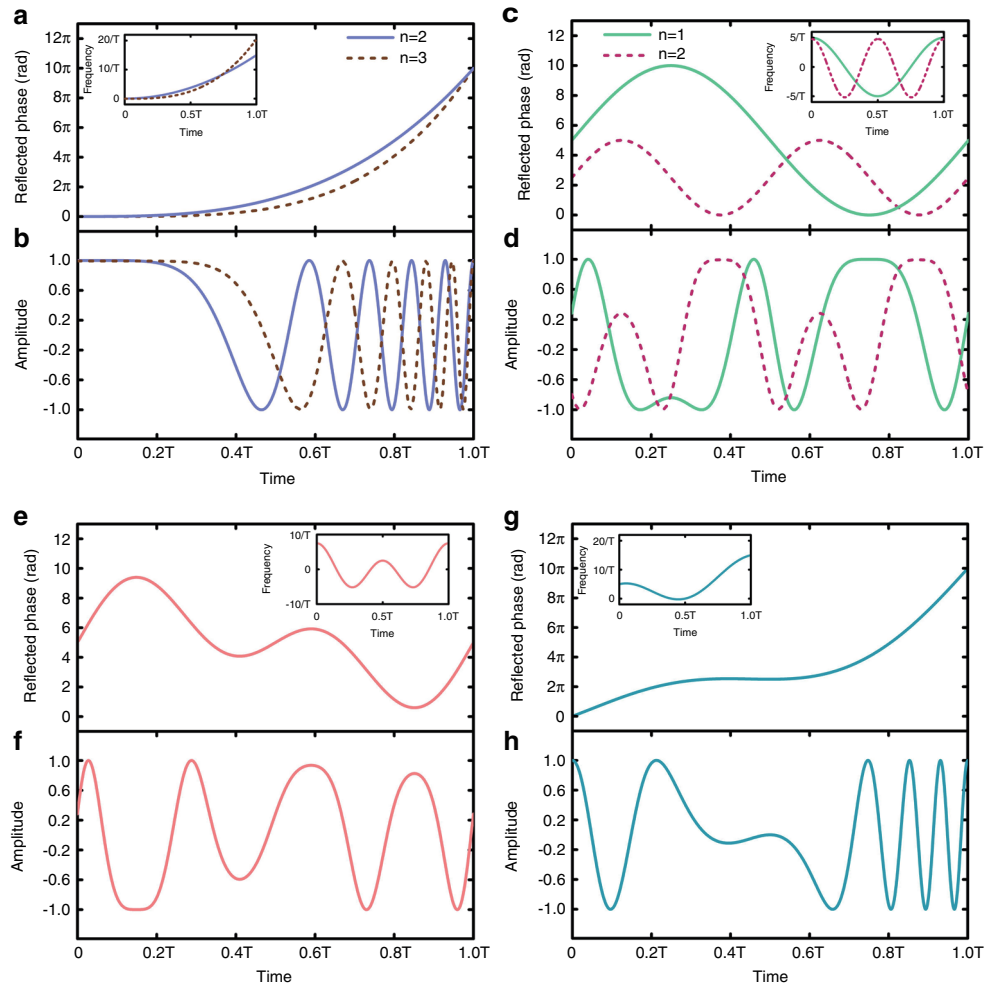
Fig. 3 Generations of nonlinear FMCW signals based on STCM with nonlinear periodic phases. a, c, e, g , Reflection phase responses \varphi_0(t) for Polynomial FMCWs under two different power index n ( a ), Sinusoidal FMCWs under two different coefficient n ( c ), Double sinusoidal FMCW ( e ), and S-shaped FMCW ( g ), in which the insets of a, c, e, g show the corresponding time-frequency diagrams after down-conversions. b, d, f, h The nonlinear FMCW waveforms of the four types in baseband.
